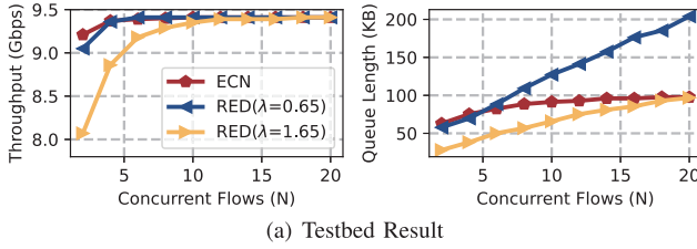
Fig. 3. RED performance with different flow concurrency levels ( N ).
