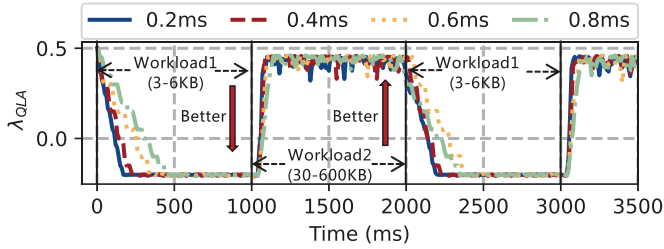
Fig. 26. [Simulation] \lambda_{QLA} of different T_{QLA} .
