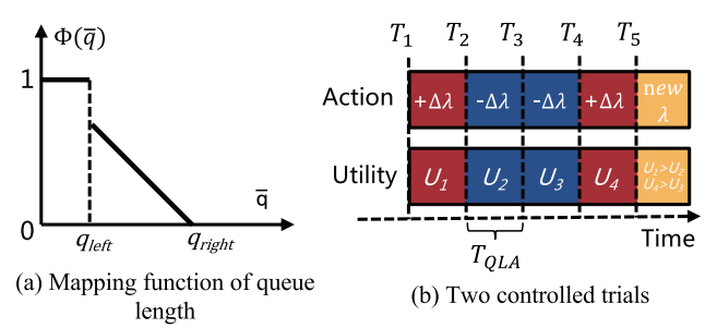
Fig. 10. Design details of QLA.
