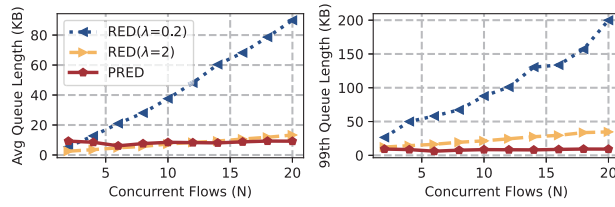
(a) Different flow concurrency levels
