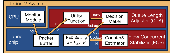
(b) Hardware architecture of PRED on Tofino 2.
